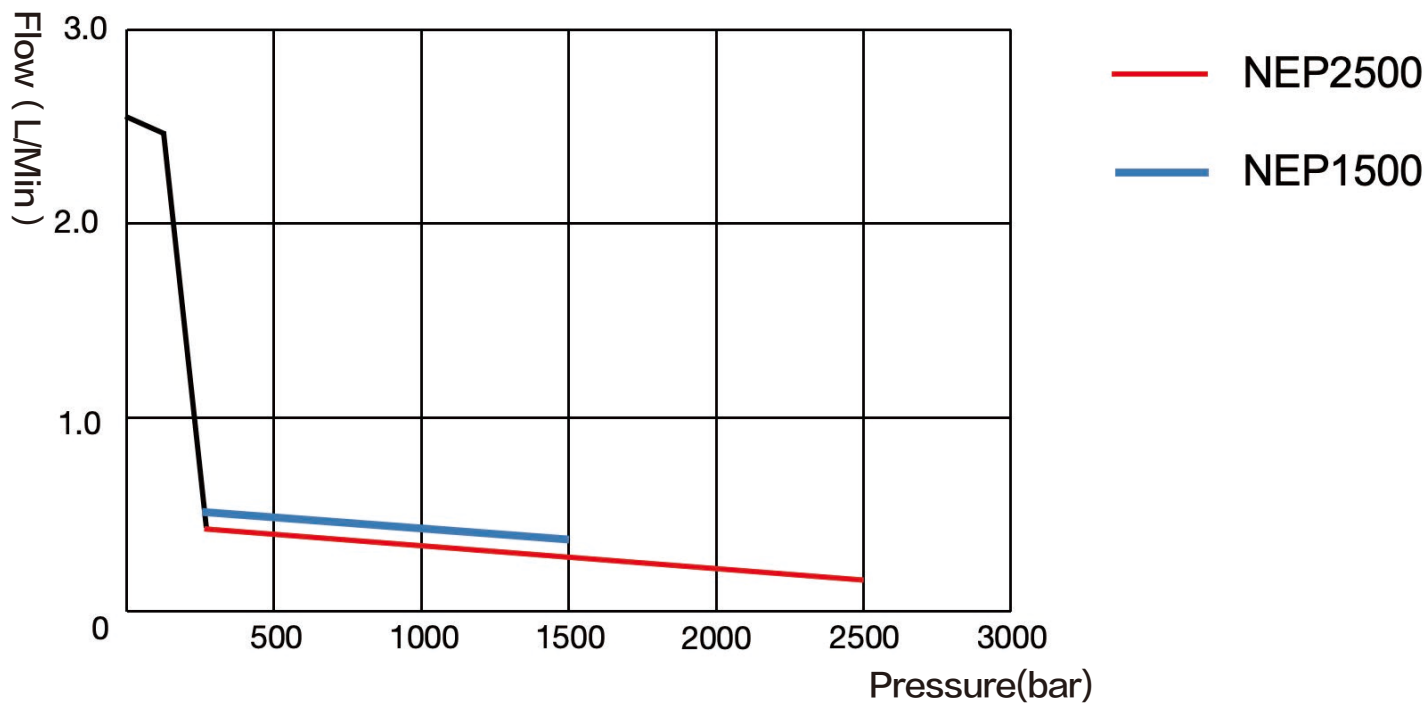
▼ NEP Flow-Pressure Curve :
